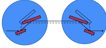
Figure 5: Optical layout of a four-crystal monochromator [?].
