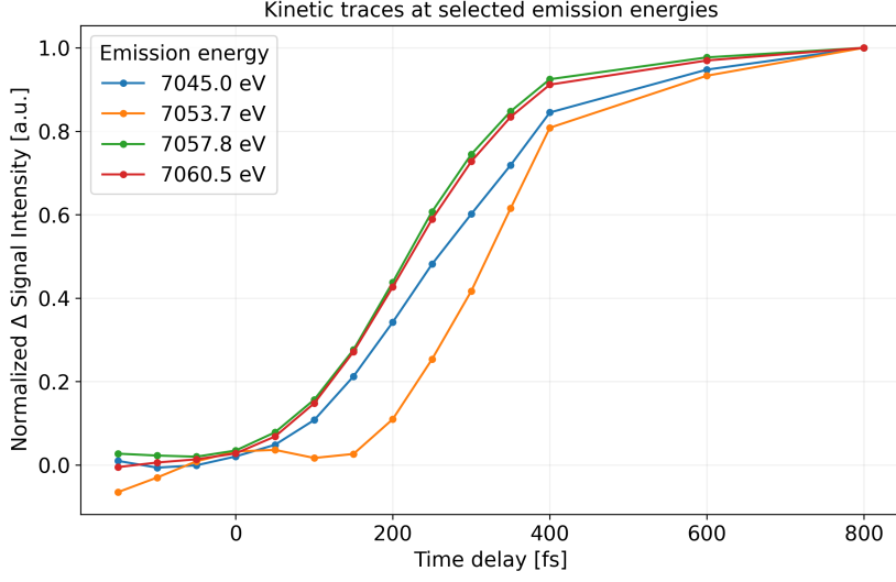
Figure 19: Kinetic traces at selected emission energies.
